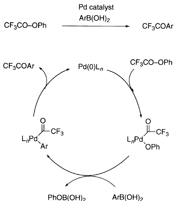
Scheme 1. Catalytic cycle for the formation of trifluoromethyl ketones.
